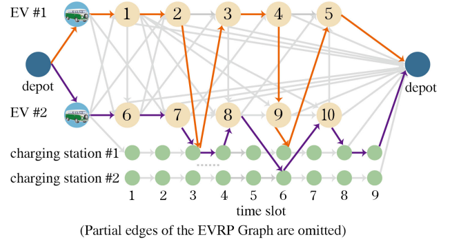
Fig. 2. The EVRP graph, with a single pair of origin and destination depots, 2 charging stations (#1 and #2), 2 EVs (#1 and #2) and 10 customers. The two depot nodes are v_o and v_d , nodes with EV are virtual vehicle nodes, the brown nodes and green nodes are task nodes and charging nodes, respectively. Some edges of the graph are omitted due to simplification.
