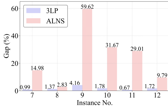
Fig. 4. The optimality gap of EVRP-3LP algorithm and ALNS algorithm.
