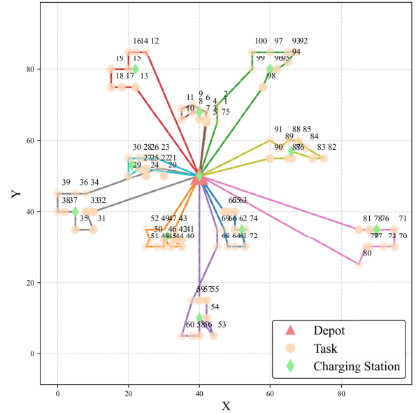
Fig. 1. A schematic diagram illustrating the Electric Vehicle Routing Problem (EVRP). The diagram showcases a scenario involving 10 electric vehicles, 100 transportation tasks, and 11 charging stations. Solid lines represent the planned routes for the vehicles, with each color indicating the route of a specific vehicle.
